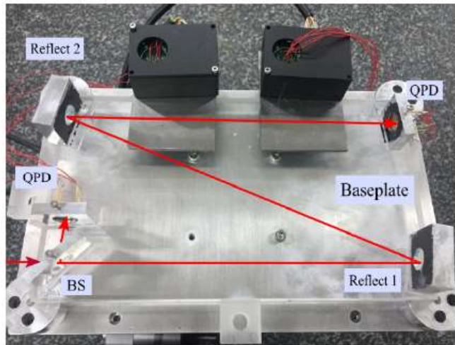
Fig. 12. Photograph of CQP.
