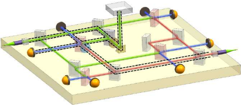
Fig. 3. Composition of laser interferometry system.
