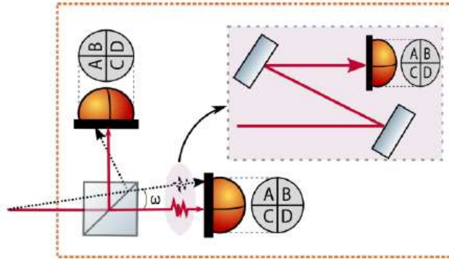
Fig. 11. Concept of CQP.
